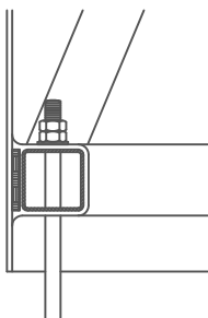
2 S1 ANCHOR DETAIL
