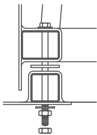
3 S1 BOLTING DETAIL
