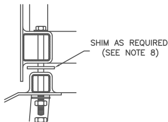
4 S1 BOLTING DETAIL
