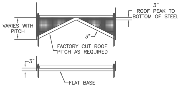
6 S1 BASE DETAIL
