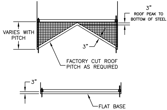
5 S1 BASE DETAILS
