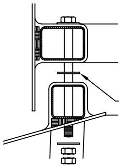
3 S1 BOLTING DETAIL
