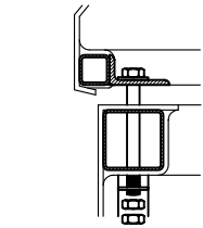
5 BOLTING DETAIL S1
