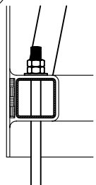
2 ANCHOR DETAIL S1
