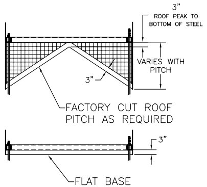
6 BASE DETAILS S1
