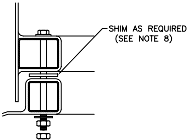
3 BOLTING DETAIL S1
