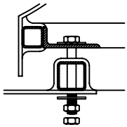
4 BOLTING DETAIL S1
