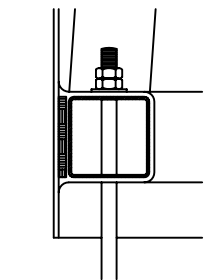
2 ANCHOR DETAIL S1
