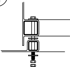
4 BOLTING DETAIL S1
