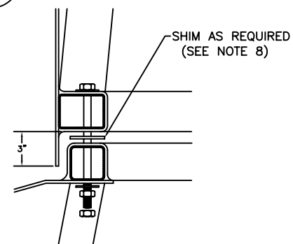
3 BOLTING DETAIL S1
