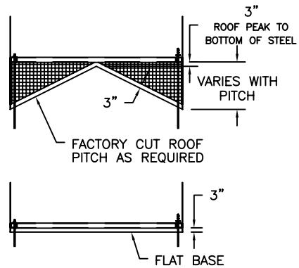
6 BASE DETAILS S1
