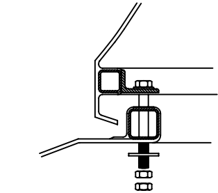
4 S1 BOLTING DETAIL
