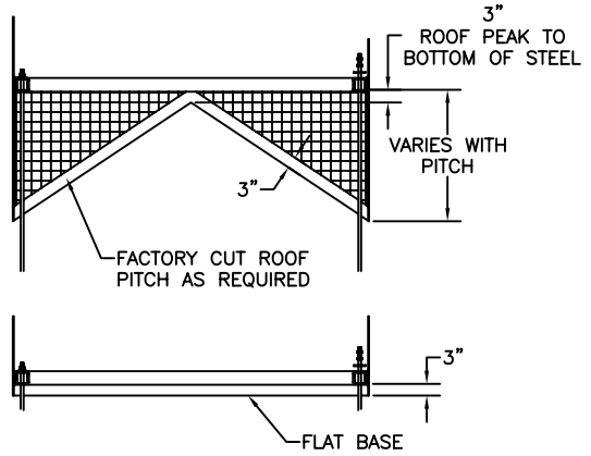
5 S1 BASE DETAILS
