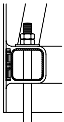
3 S1 BOLTING DETAIL
