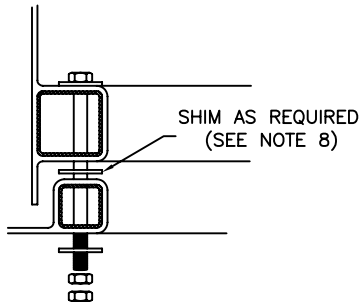
3 S1 BOLTING DETAIL
