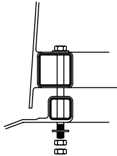
4 S1 BOLTING DETAIL
