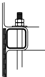
2 S1 ANCHOR DETAIL
