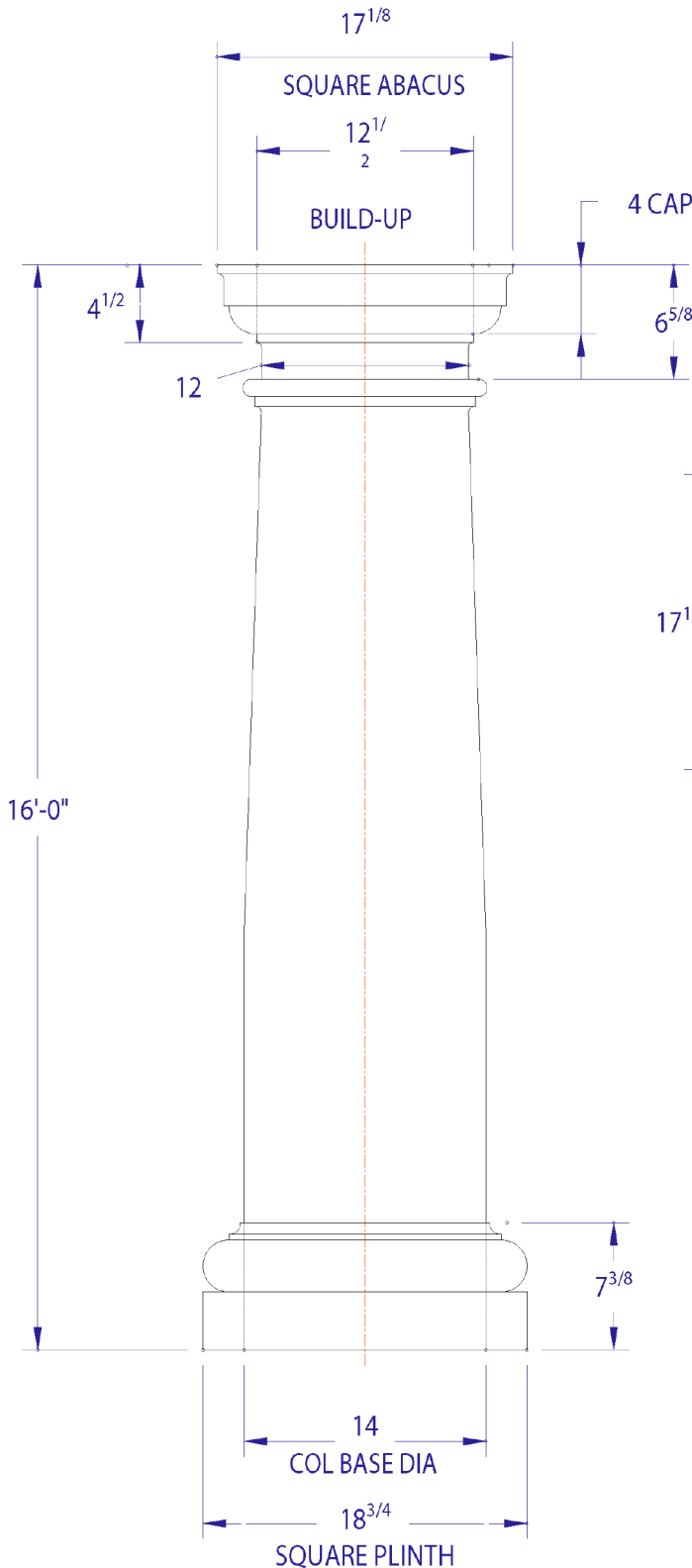
14" DIAMETER COLUMN - TUSCAN
