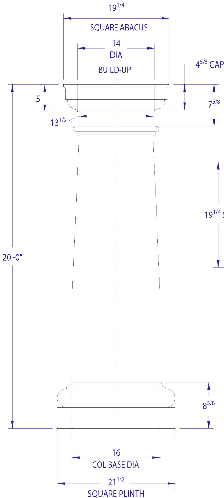
16" DIAMETER COLUMN - TUSCAN
